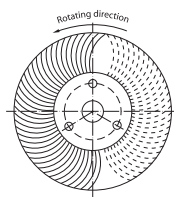
Cut design 1 Right-hand cutting, usable both sides
