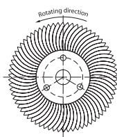
Cut design 4 One-sided cutting with teeth on periphery
